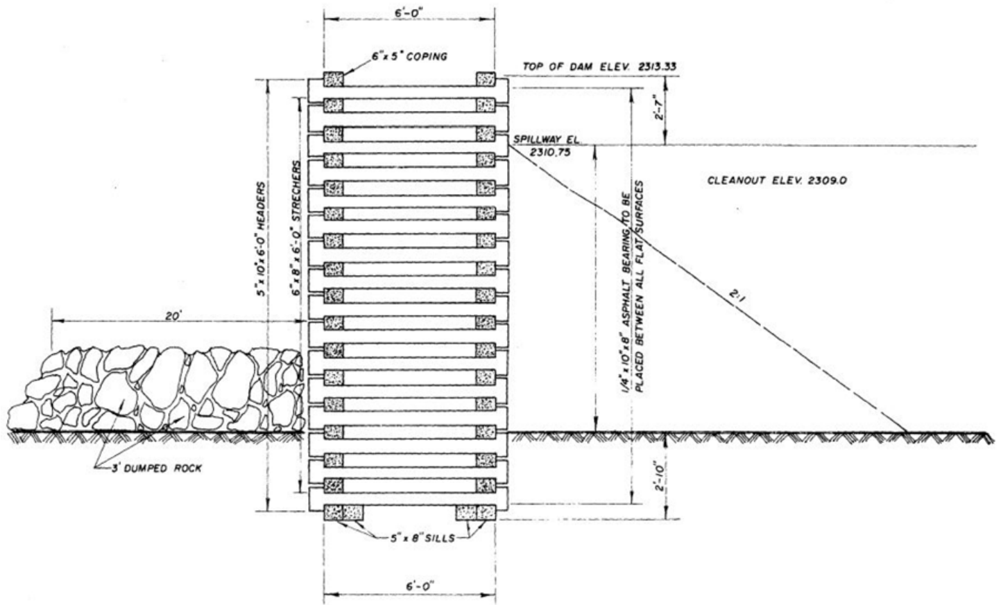
CROSS SECTION VIEW OF CRIB DAM NO.2
