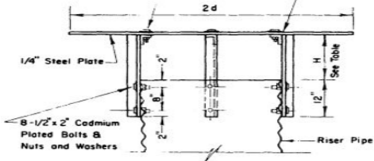
SECTION AT CENTER
