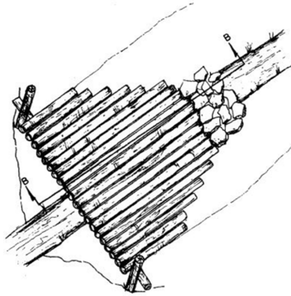
LOG & POLE SILT STRUCTURE
