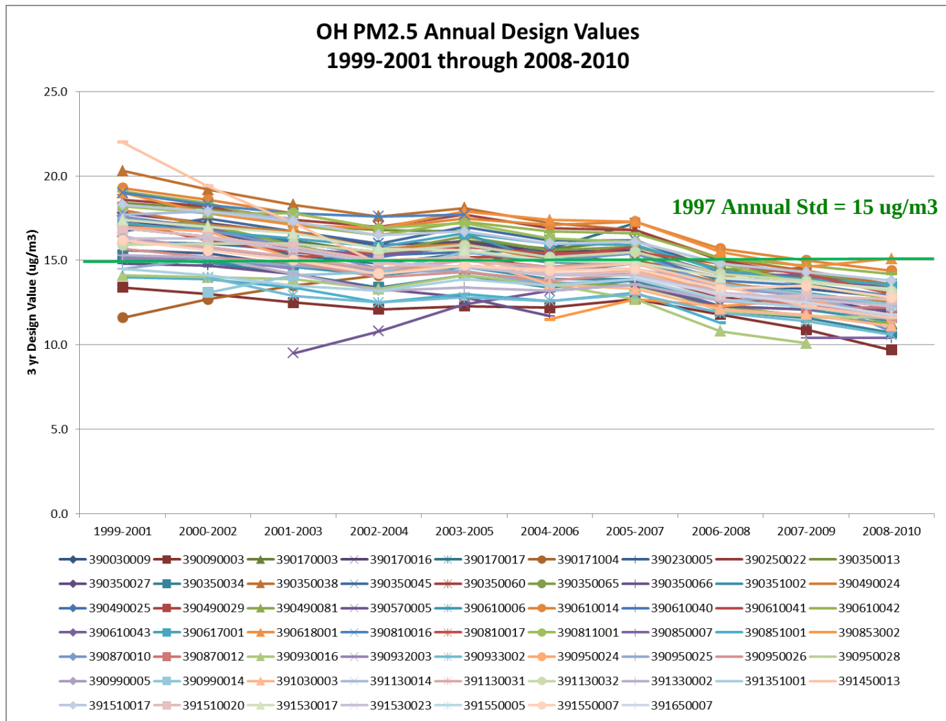
Figure 3: Ohio PM 2.5 Annual Design Values, 1999-2001 through 2007-2009.
