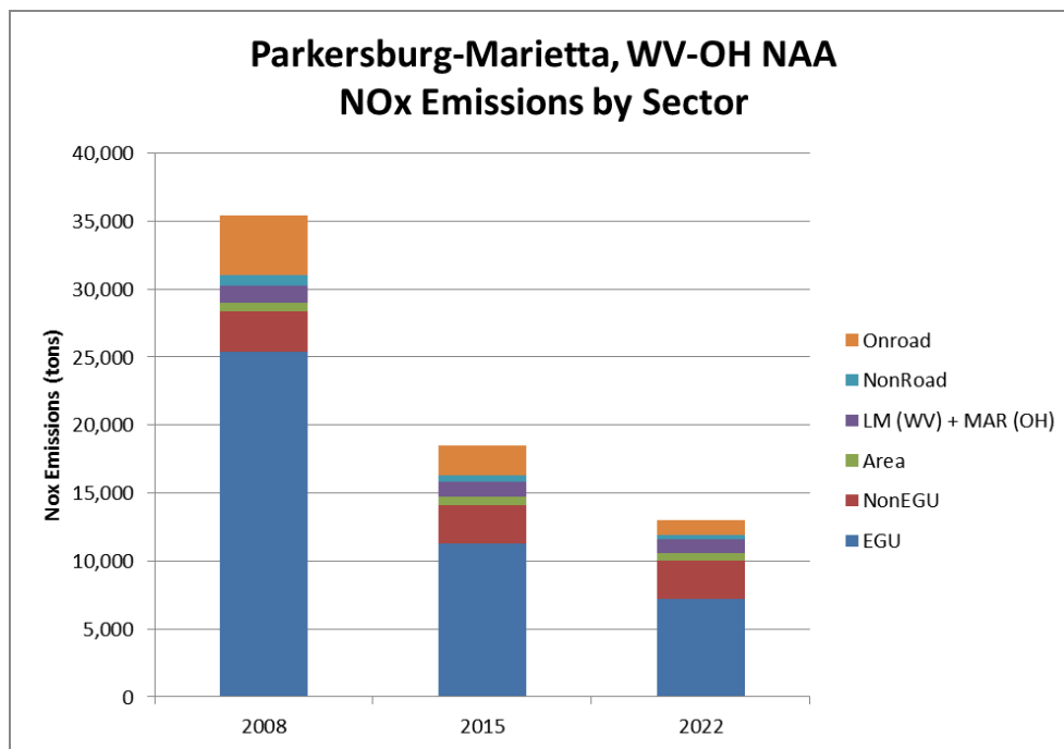
Figure 7: Parkersburg-Marietta, WV-OH NO x Emissions by Sector
