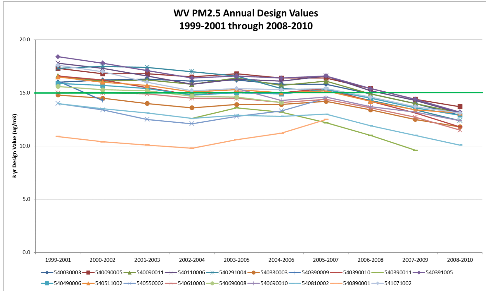
Figure 2: West Virginia PM 2.5 Annual Design Values, 1999-2001 through 2008-2010.
