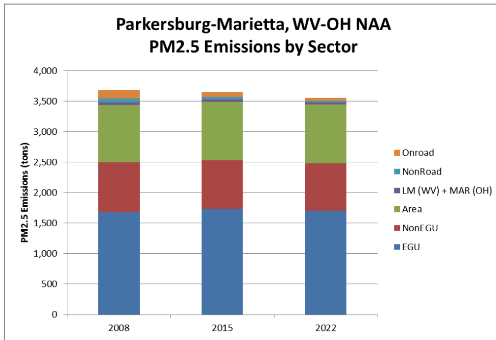
Figure 8: Parkersburg-Marietta, WV-OH NAA PM 2.5 Emissions by Sector
